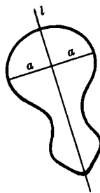
Symmetry with respect to a line l .
