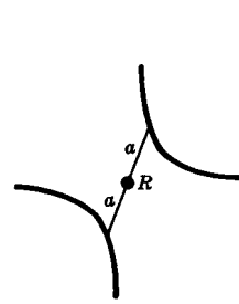
Symmetry with respect to a point R .
