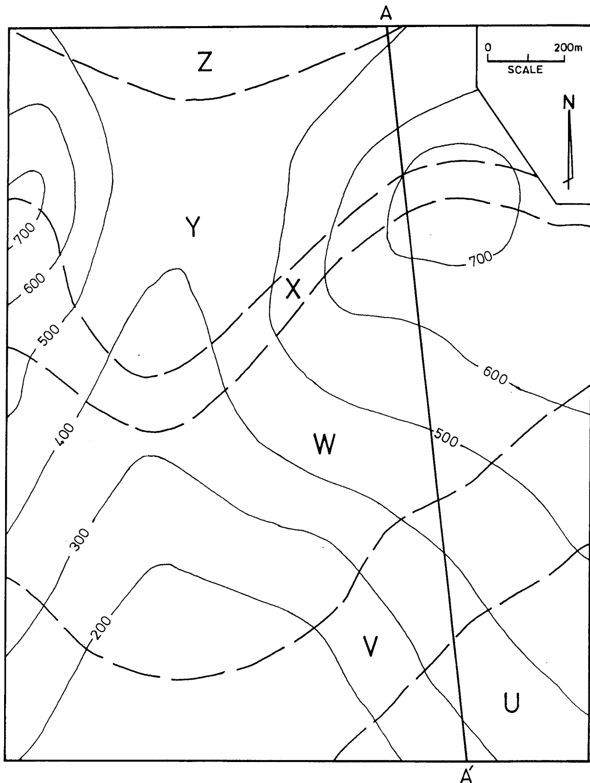
Fig. 2: Geological map
