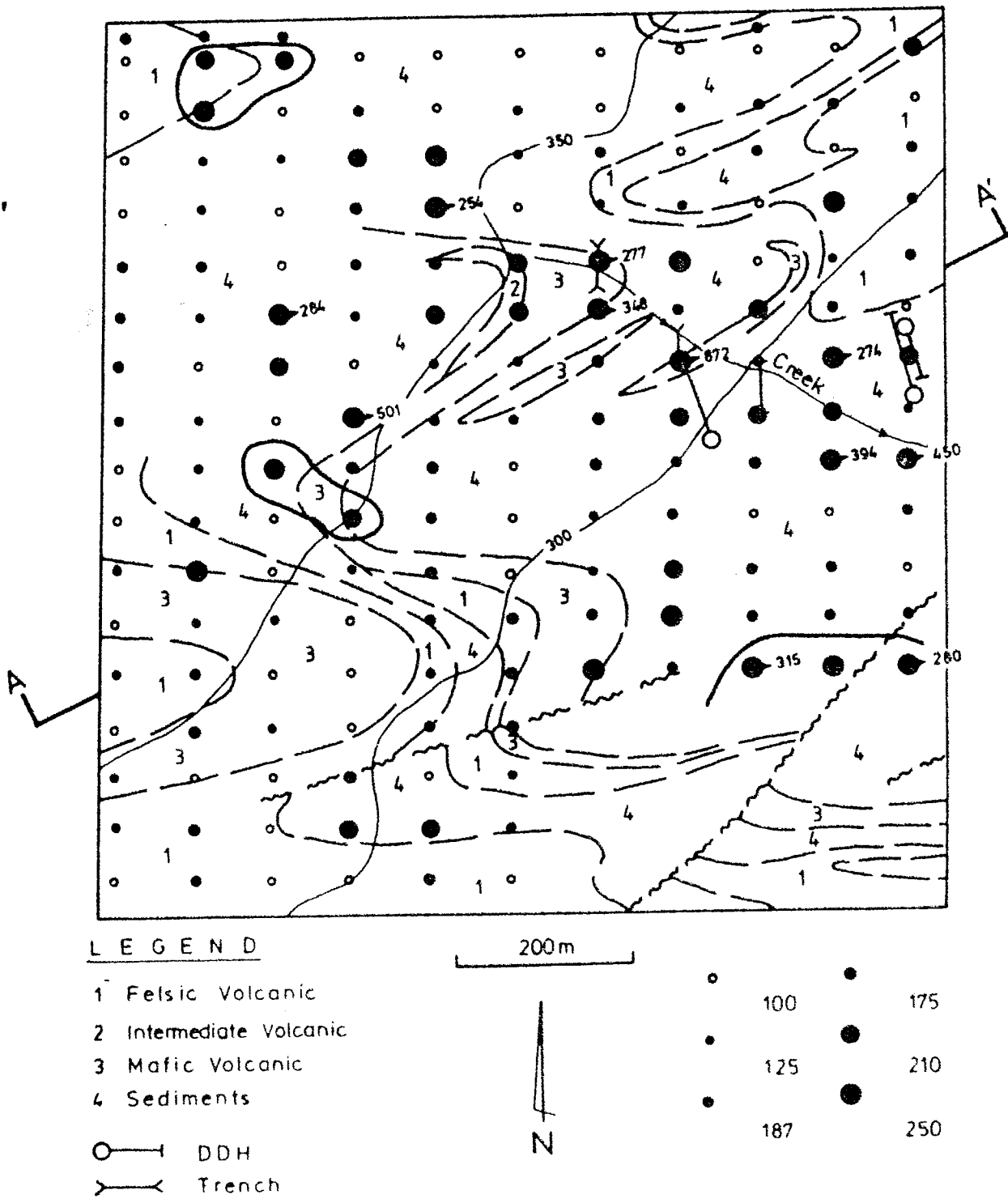
Figure 1 A geochemical map showing geology, topography, Zinc values and trench / drill holes from a public domain map
