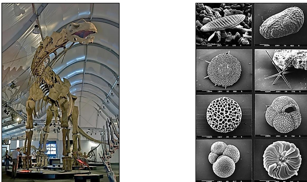
Figure 4.2. Argentinosaurus from Argentina, the largest type of dinosaur known so far, and scanning electron microscope (SEM) images of tiny marine microfossils
