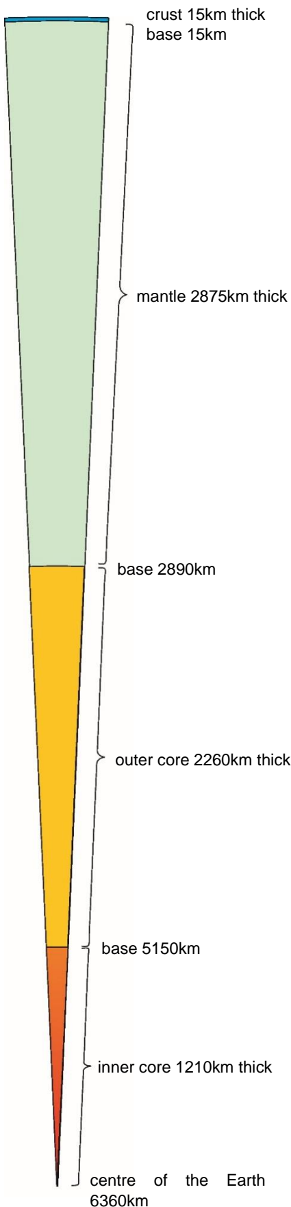
Figure 4.9. Cross-section of the Earth
