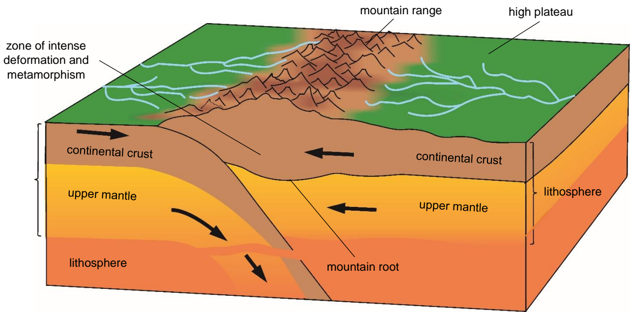
Figure 4.31. Collision of the Indian plate with the Eurasian plate, producing the Himalayan mountain chain
