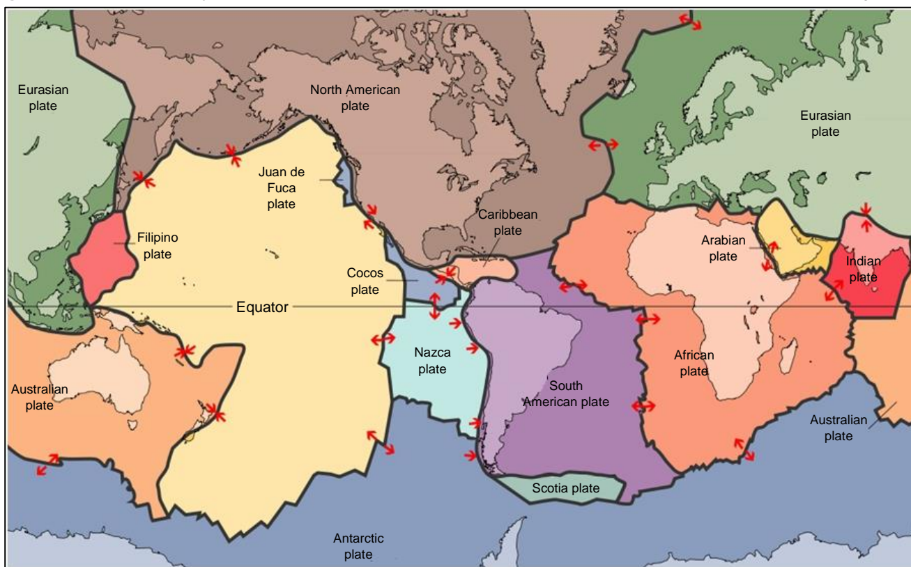
Figure 4.35. The Earth's major tectonic plates; the red arrows show the directions of plate movement at the plate margins
