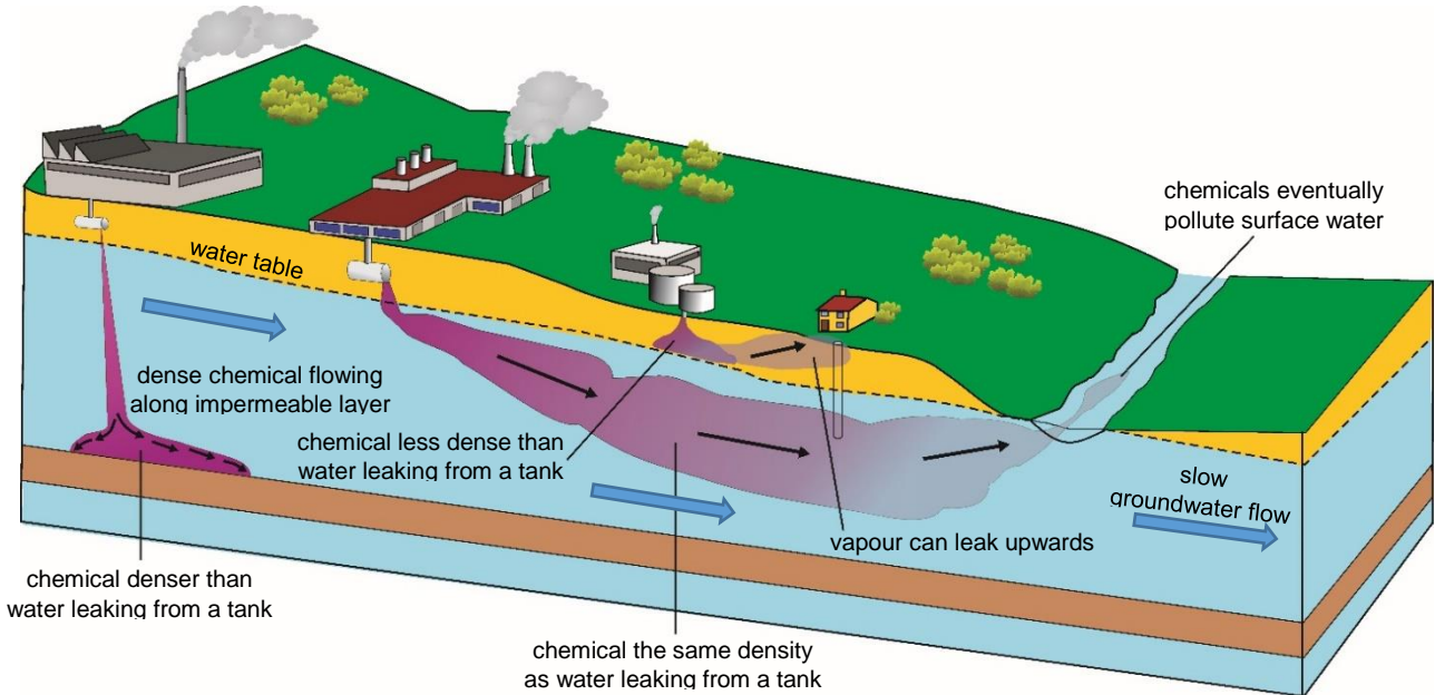
Figure 4.38. Plumes of groundwater pollution
