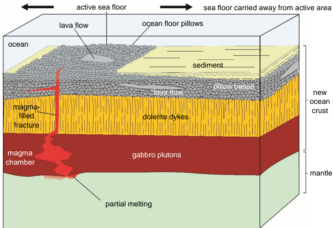
Figure 4.6. Igneous bodies in oceans
