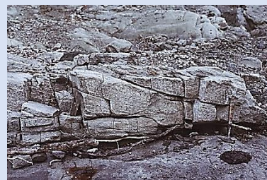
Cross-bedded Jurassic sandstone, showing flow of the ancient river from the West (left)
