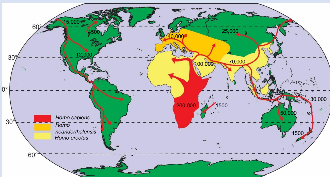
The spread of early human groups across the world, with spreading dates: first – Homo erectus ; second – Homo neanderthalensis ; third – Homo sapiens
