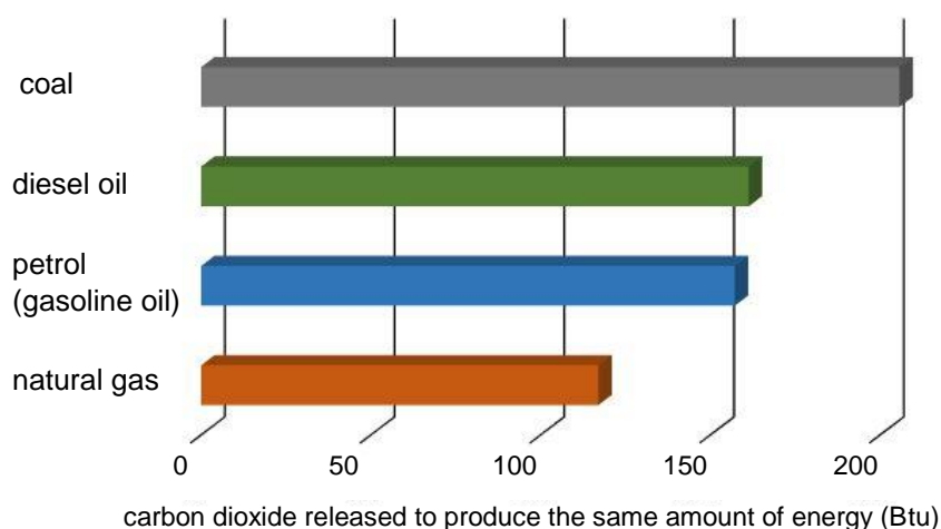
Figure 5.7. The amounts of carbon dioxide released by the burning of different fossil fuels to produce the same amount of energy
