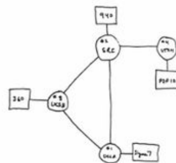
THE ARPANET NETWORK
