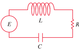
FIGURE 4.4.2 LRC-series circuit
