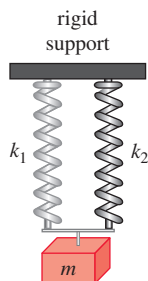
FIGURE 3.8.5 Parallel springs
