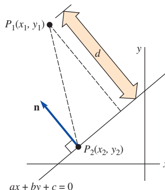
FIGURE 7.3.14 Distance d in Problem 53
