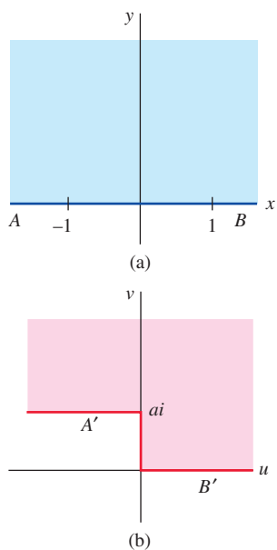
FIGURE 20.4.5 Image of upper half-plane in Example 2
