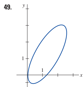
FIGURE 1.1.5 Graph for Problem 49
