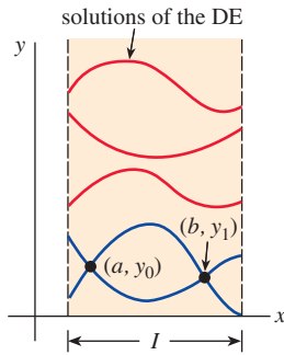
FIGURE 3.1.1 Colored curves are solutions of a BVP
