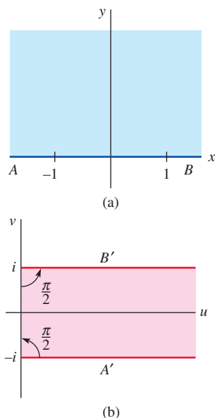
FIGURE 20.4.4 Image of upper half-plane in Example 1
