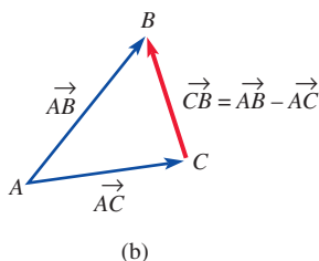
FIGURE 7.1.5 Vector \overrightarrow{CB} is the difference of \overrightarrow{AB} and \overrightarrow{AC}
