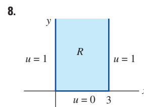
FIGURE 20.5.11 Dirichlet problem in Problem 8
