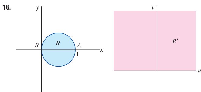
FIGURE 20.2.13 Regions R and R' for Problem 16
