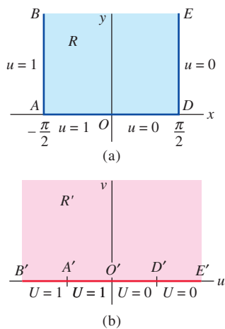
FIGURE 20.2.5 Image of semi-infinite vertical strip in Example 6
