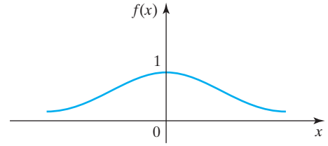
FIGURE 10.8 The hump function.
