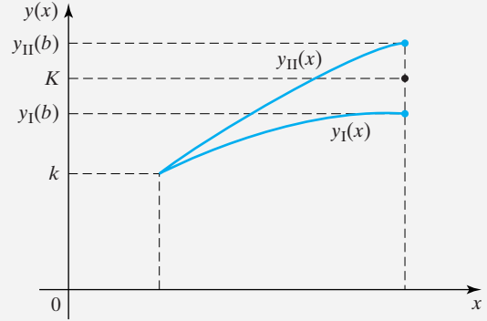
FIGURE 19.12 The two solutions y_I(x) and y_{II}(x) .
