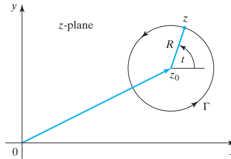
FIGURE 14.6 The circle \Gamma .
