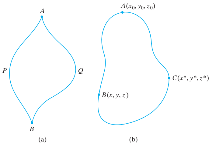
FIGURE 18.14 (a) Two paths joining A to B . (b) A loop containing a fixed point A .
