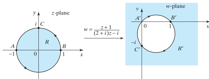
FIGURE 17.8 The mapping \frac{z+1}{(2+i)z-i} .
