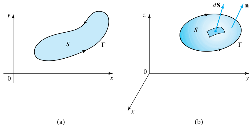
FIGURE 12.2 (a) A plane oriented surface. (b) A general oriented surface in space.
