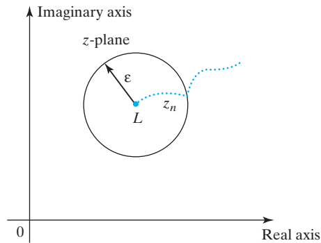
FIGURE 15.1 A convergent complex sequence \{z_n\} with limit L .
