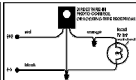
48, 24 & 12 VDC For DC Wiring Applications Only Color Coded Leads Red - (+) Black - (-) Orange - Load
