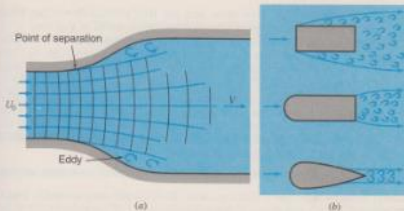
Figure 4.13 Separation in diverging flow. (a) Eddy formation in a diverging channel. (b) Turbulent wakes.
