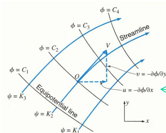
Figure 14.10 Flow net.
