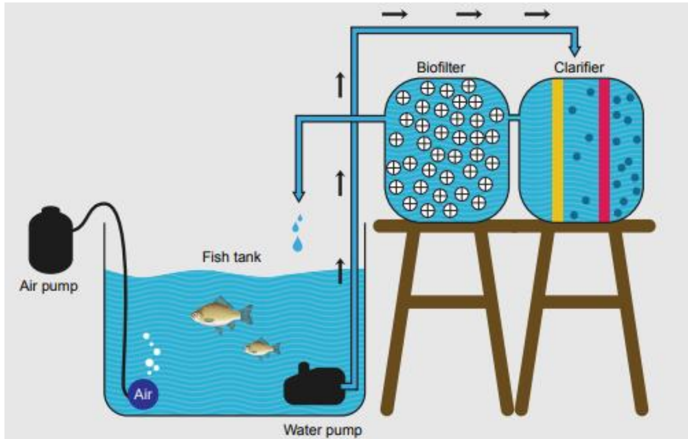
Basic Recirculating aquaculture system set up
